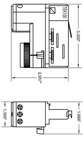
TA2S Specification Grade 120V, 2 circuit Track Adapter.
