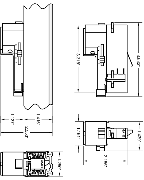
TA3 Specification Grade 120V, 3 circuit Track Adapter.
