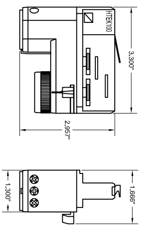
HTA2 Specification Grade 277V, 2 circuit Track Adapter.
