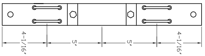
DOUBLE PIPE HANGER FOR CABLE
