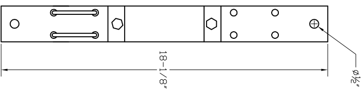
DOUBLE PIPE HANGER FOR CABLE
