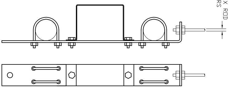
DOUBLE PIPE HANGER FOR THREADED ROD
