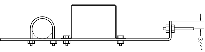
SINGLE PIPE HANGER FOR THREADED ROD
