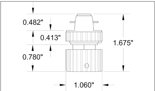
99-507 Mechanical adapter for all E-Series track.
