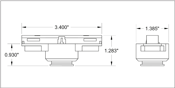
STAI Track adapter for E-Series 1-Circuit data track. 120V.
