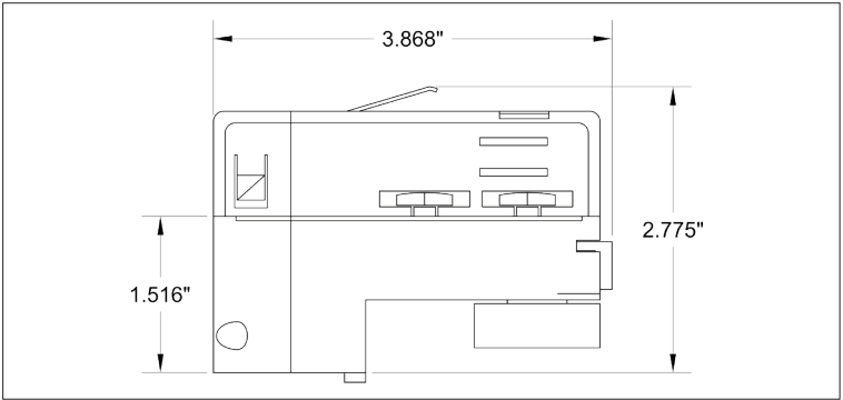
HDT2 Track adapter for SpecTrack 2-Circuit data track. 277V.
