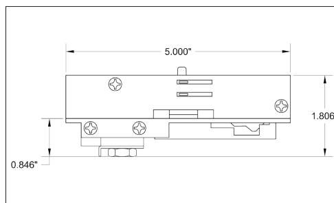
FIT LSI™ compatible 2-circuit track adapter. 120V
