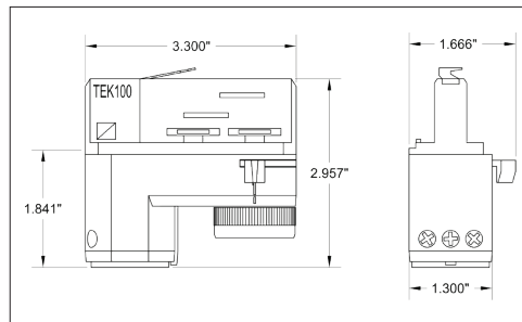
TA2 Track adapter for G-Series specification grade 2-Circuit track. 120V.
