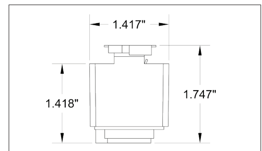
AD12 JUNO™ compatible track adapter. 120V.
