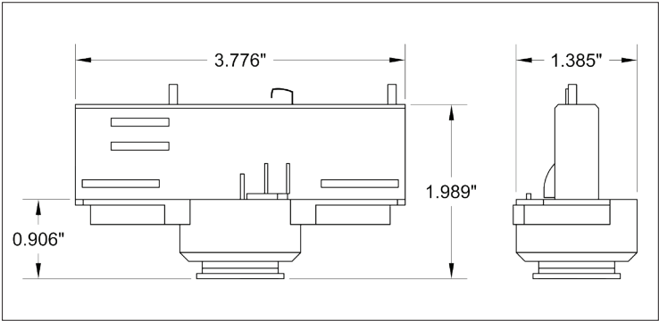
STA Track adapter for E-Series 2-Circuit Data Track. 120V.
