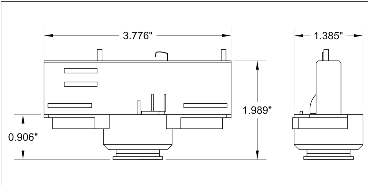
HSTA Track adapter for E-Series 2-Circuit Data track. 277V.
