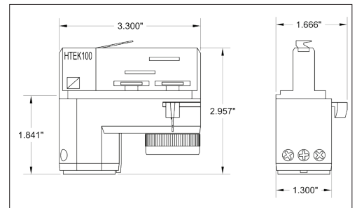
HTA2 Track adapter for G-Series specification grade 2-Circuit track. 277V.
