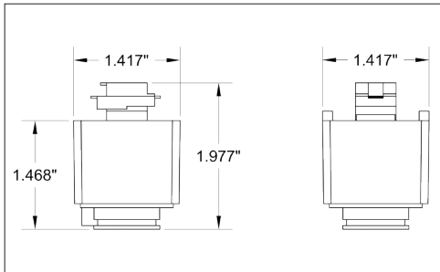
AD1 Track adapter for commercial grade 1 and 2-Circuit track. This adapter is Halo™ and Times Square compatible. 120V.
