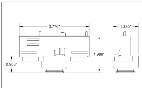
TE2 Track adapter for E-Series specification grade 2-Circuit track. 120V.
