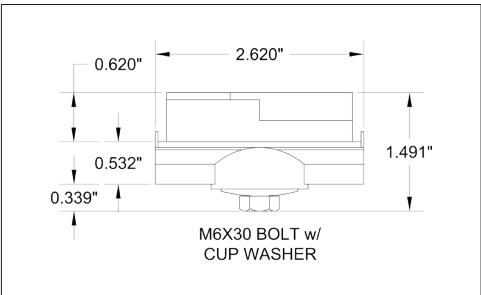
W-499-1 Mechanical adapter with M6 bolt and belleville washer for all G-Series track.
