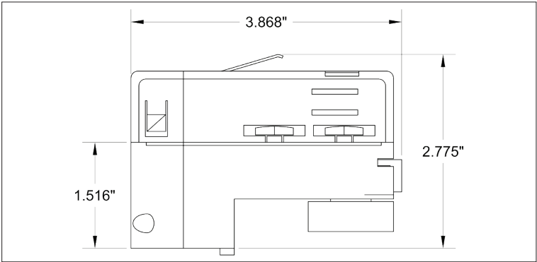
DT2 Track adapter for SpecTrack 2-Circuit data track. 120V.
