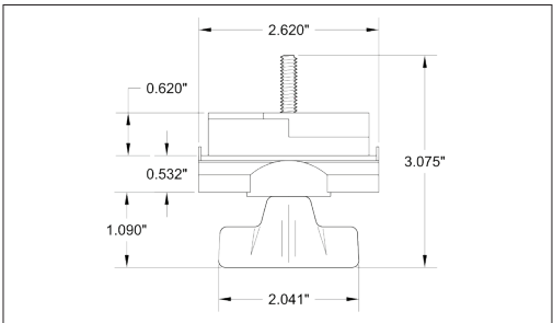
W-449 Mechanical adapter with T-Handle for all G-Series track.
