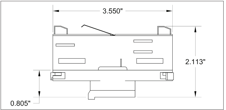
GAC Track adapter for Pulse 3-Circuit data track. 120V.
