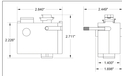
T1 Track adapter for commercial grade 1 and 2-Circuit track. This adapter is Halo™ and Times Square compatible. 120V.
