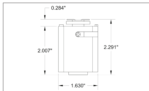
AD14 TYPE 2 LIGHTOLIER™ compatible track adapter with lever. 120V.
