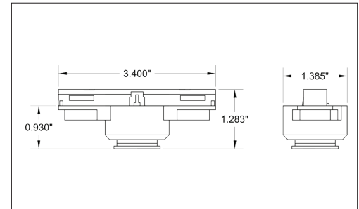
TAI Track adapter for E-Series specification grade 1-Circuit track. 120V.
