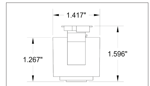
G1 Track adapter for GES Series 1-Circuit track. 120V.
