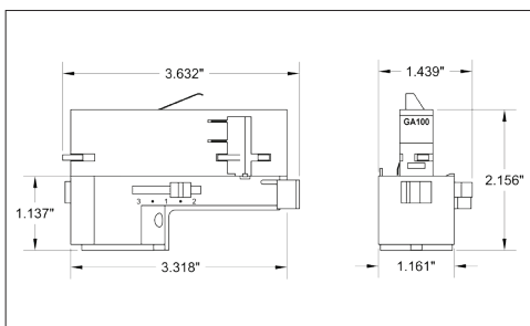
TA3 Track adapter for G-Series specification grade 3-Circuit track. 120V.
