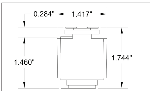
AD14 TYPE 1 LIGHTOLIER™ compatible track adapter. 120V.
