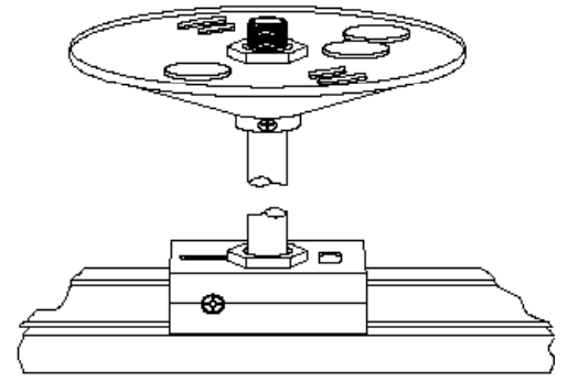
SGM4 4" Pendant Clip For positioning over end feed. For aircraft cable or 3/8" stem mounting. Can be used for electrical connection to the track.
