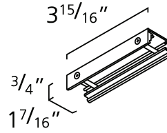
SGM4 4" Pendant Clip For positioning over end feed. For aircraft cable or 3/8" stem mounting. Can be used for electrical connection to the track.
