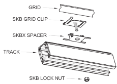
SKBX 12 Grid mounting clip.
