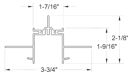
FTPX Flangeless Track Sleeve
