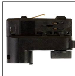
DT2 Track adapter for SpecTrack specification grade 2-circuit 120V track.
